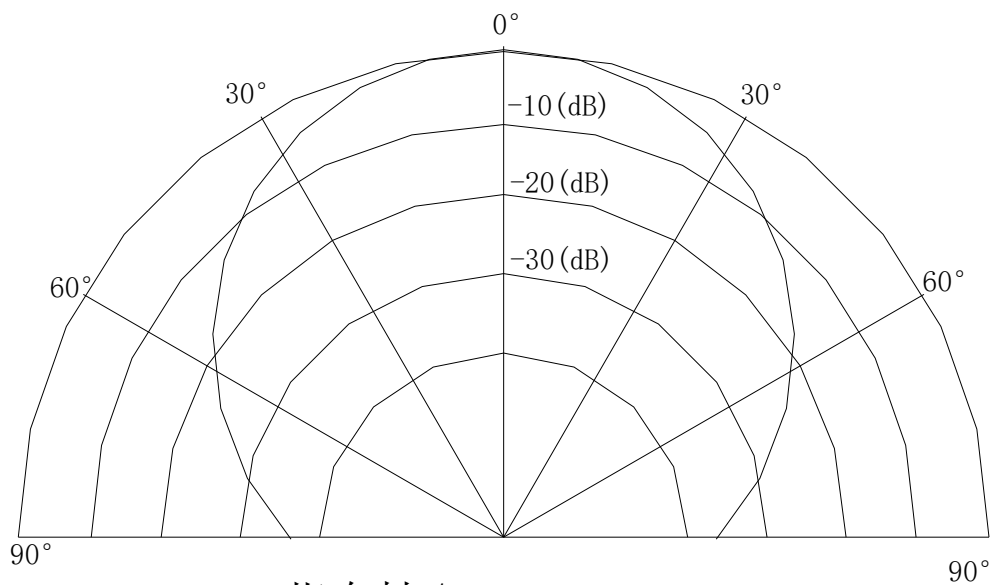
指向性/Directivity in Sensitivity
